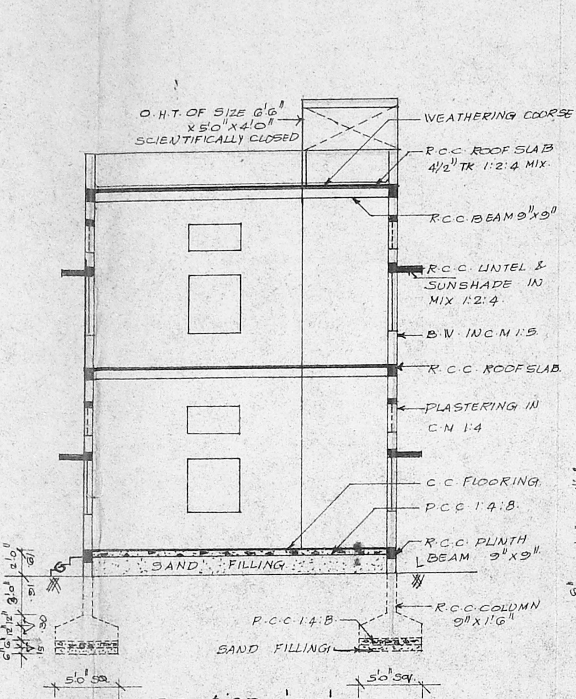
section 'aa'
